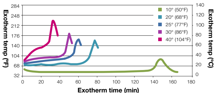
Typical Exotherm Curve for MA425 (30g mass) at Various Ambient Temperatures 5
